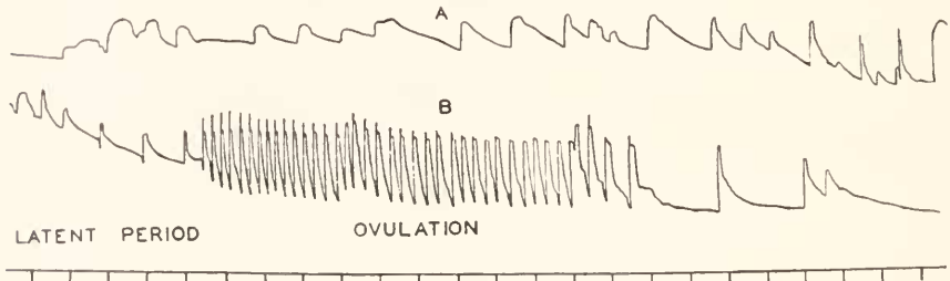
FIG. 10. Ostraea commercialis , spawning reaction of a female. A, muscular behavior during feeding. B, spawning reaction. Time interval, 1 minute (bottom line).
